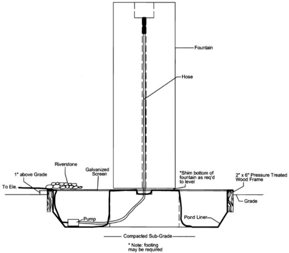
Section View
